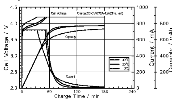
Charge characteristics
