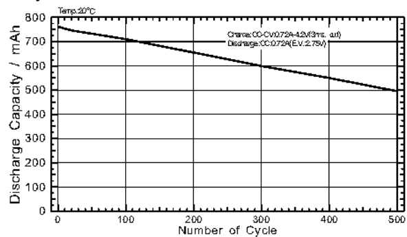
Cycle characteristics
